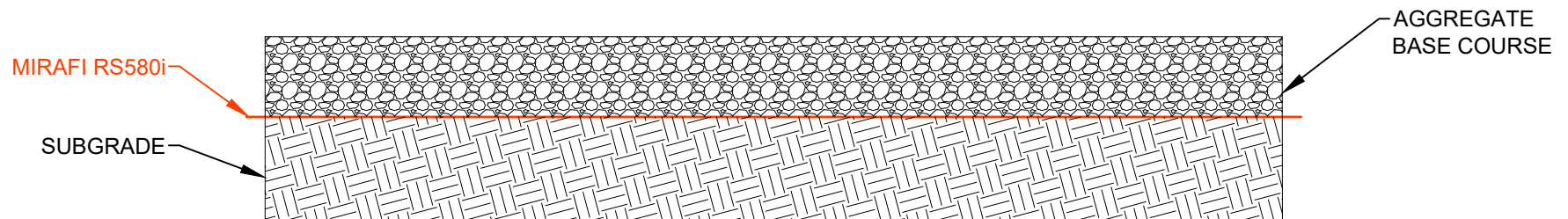
SUBGRADE STABILIZATION WITH RS580i ROAD CROSS SECTION NOT TO SCALE
