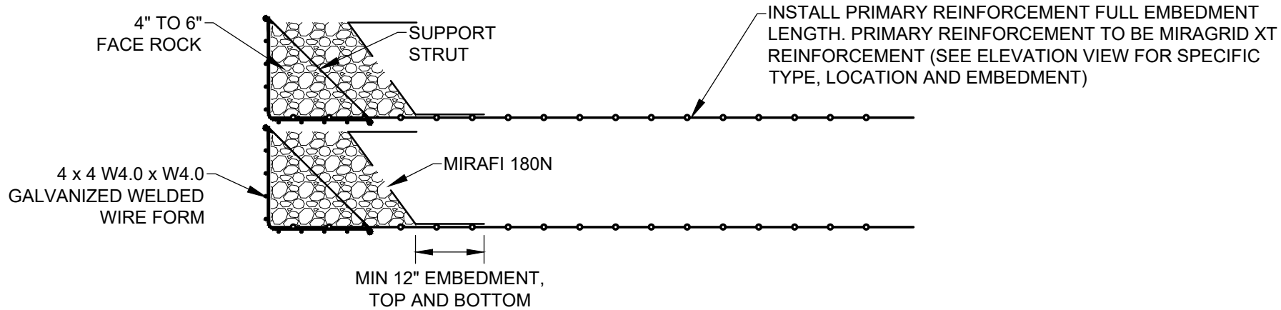
FACING DETAIL - ROCK FACE (NEAR VERTICAL) (SCALE: 1" = 2'-0")
