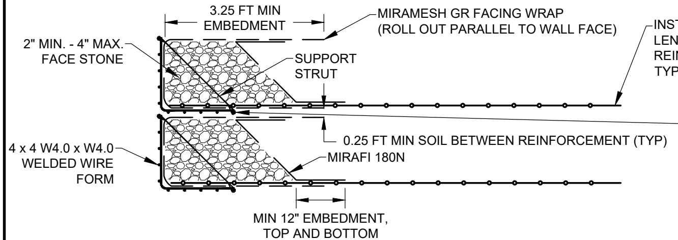
FACING DETAIL - ROCK FACE (NEAR VERTICAL) (SCALE: 1" = 2'-0")
