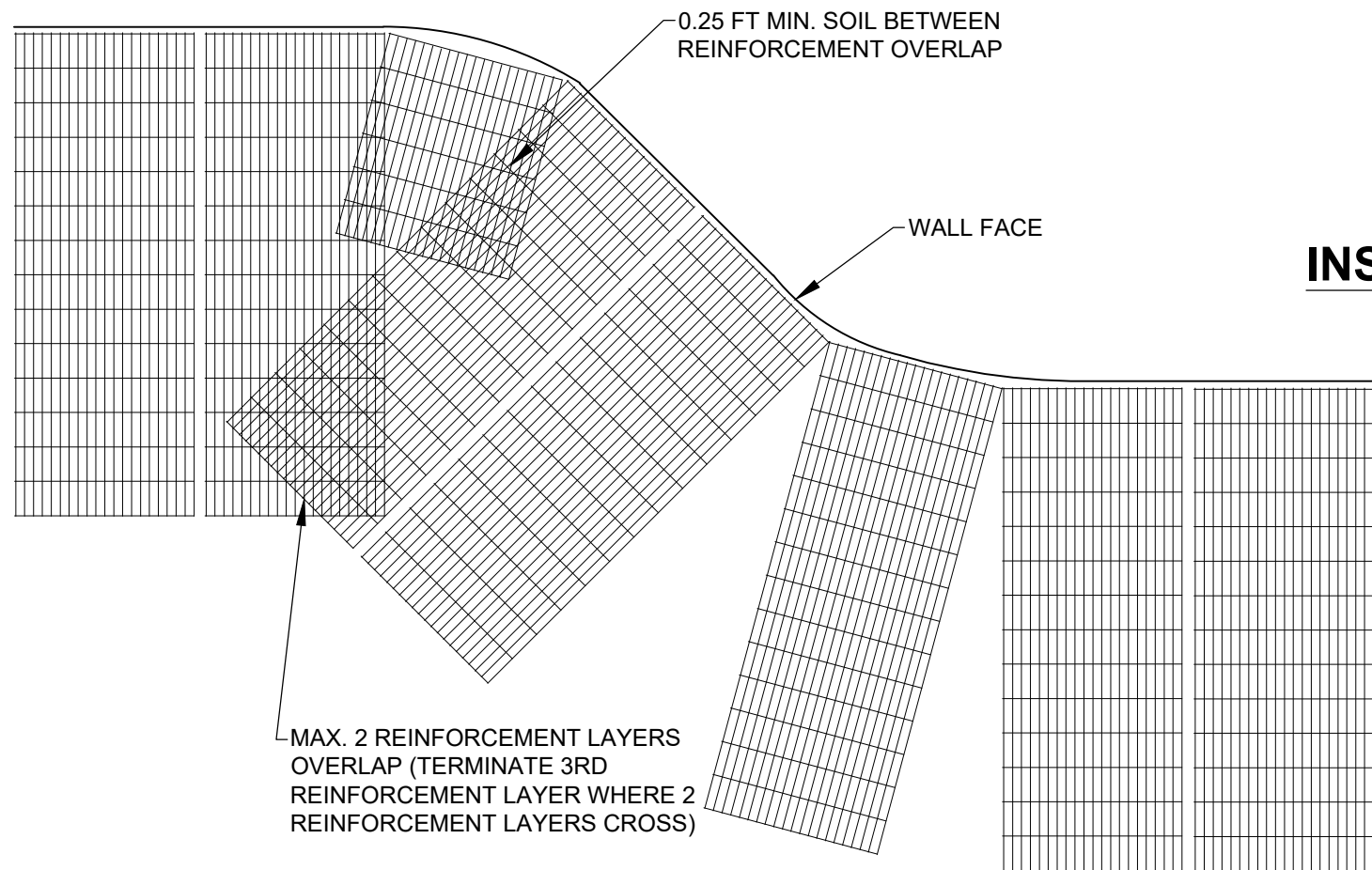
PRIMARY REINFORCEMENT PLACEMENT ON CURVES DETAIL (N.T.S.)
