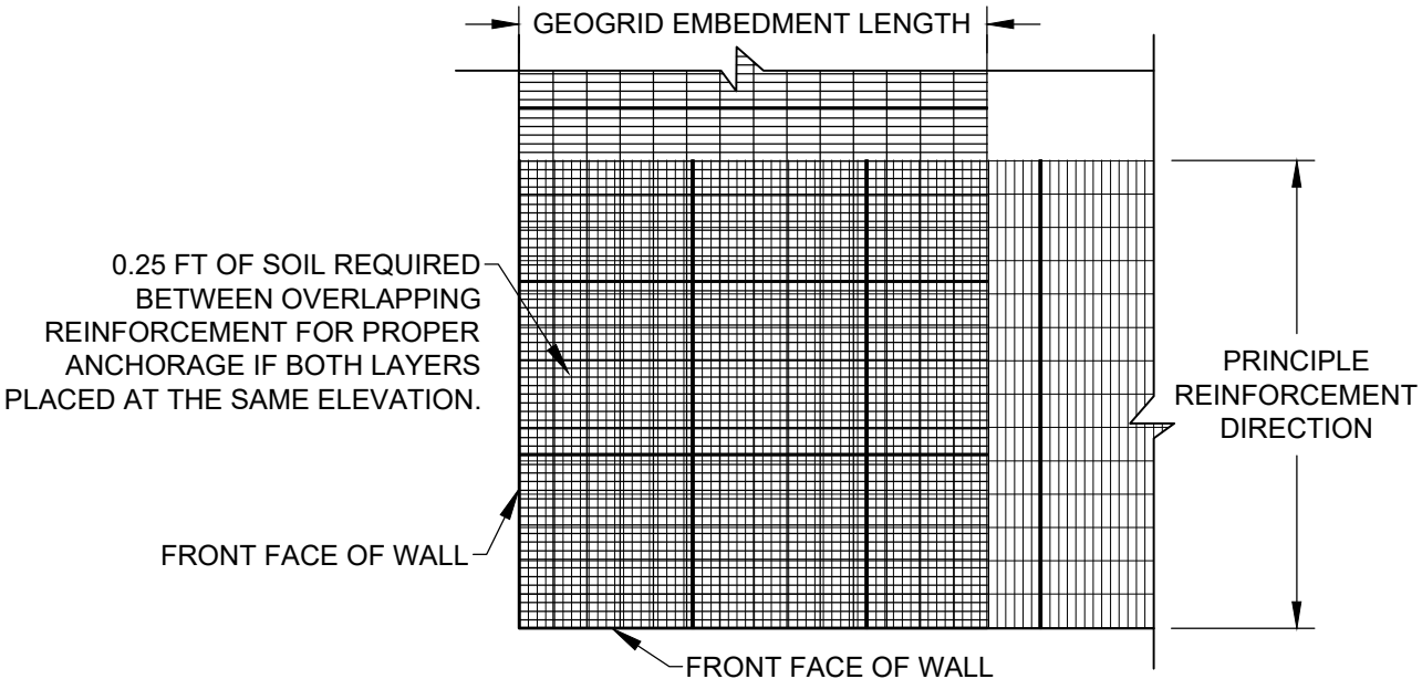
OUTSIDE CORNER REINFORCEMENT LAYOUT DETAIL (N.T.S.)
