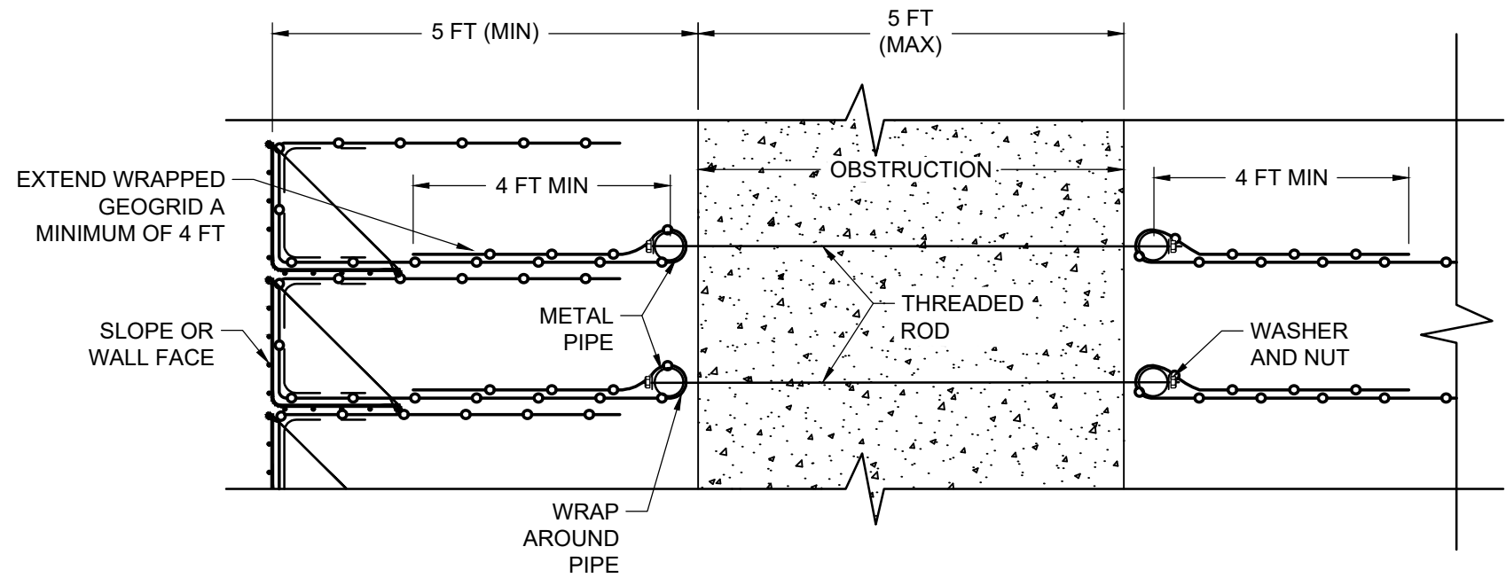
SECTION VIEW
