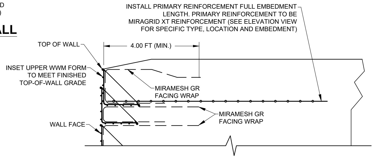
UPPERMOST WWM FORM INSET DETAIL - PERMANENT WALL (SCALE: 1" = 2'-0")
