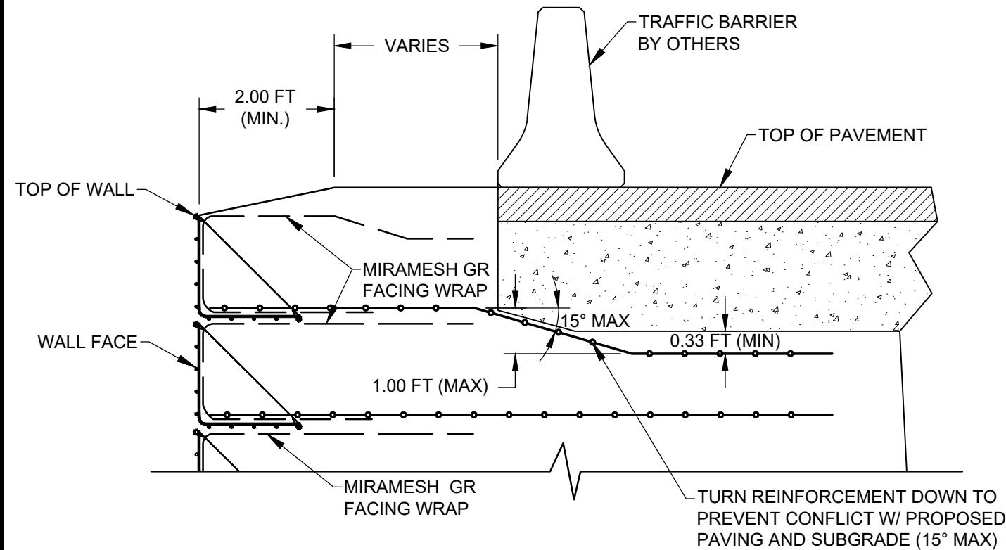
REINFORCEMENT SKEWING DETAIL - PERMANENT WALL (SCALE: 1" = 2'-0")
