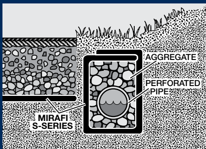
Cut-off/Interceptor Drain
