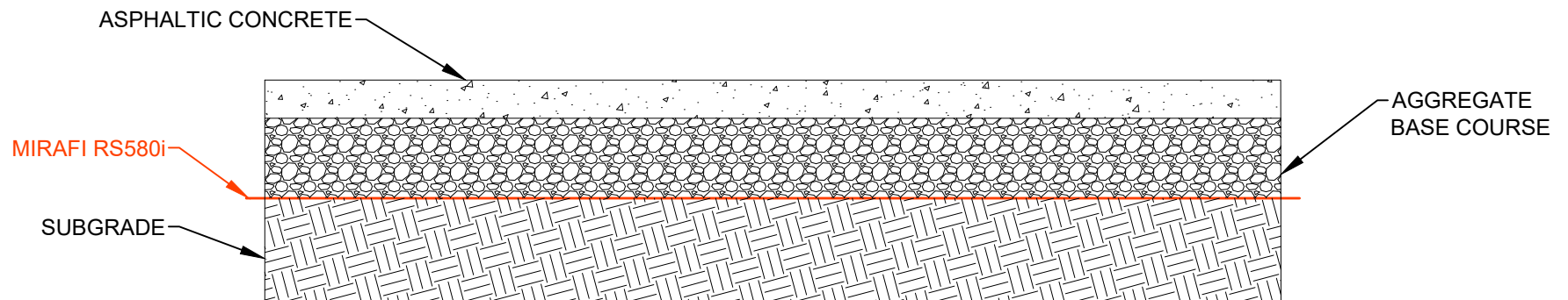
BASE REINFORCEMENT WITH RS580i ROAD CROSS SECTION NOT TO SCALE
